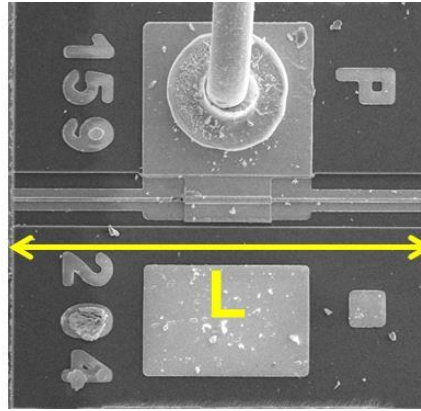
Figure 3. Measurement of the cavity length L at the SEM.
