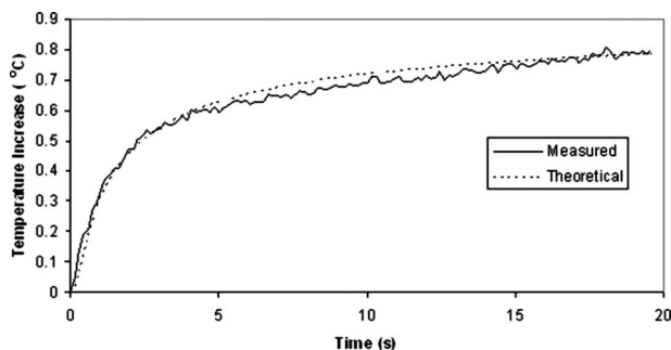
Fig. 8 Comparison of the temperature increase measured on the rear surface of a 1.35-mm-thick bone slice irradiated with 6- \mu m laser pulses scanned over a 0.5-mm radius, and the temperature predicted by Eq. (1).
