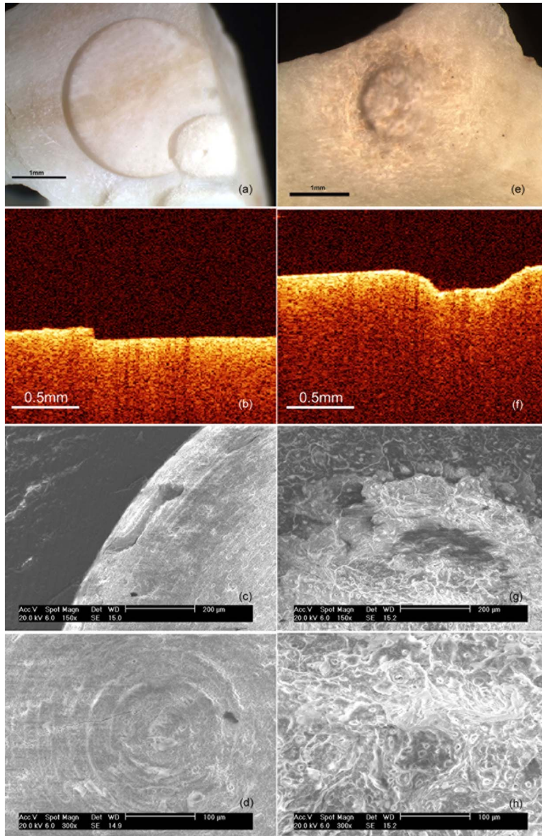
Fig. 2 Otic capsule bone ablated with femtosecond (a) to (d) and Er:YAG (e) to (h) lasers: (a) and (e), light microscopy; (b) and (f), OCT; (c) and (g), SEM×150; and (d) and (h), SEM×300.
