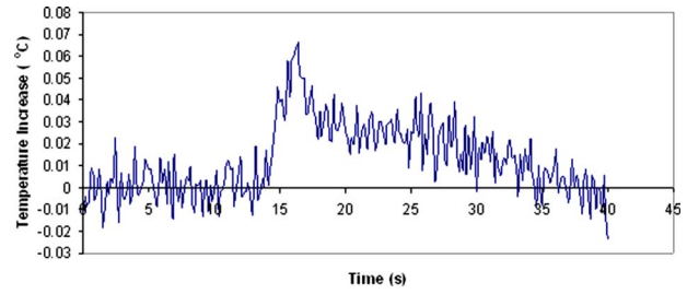
Fig. 6 Temperature increase in model ear 1 mm below the stapes for a 10- \mu\text{J} pulse scanned over 0.5 mm.
