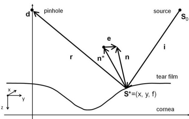
Fig. 1 Ray tracing model. The correct tear film position is determined by taking the difference of the surface and calculated normals. The required tear film position occurs when the difference is the zero vector.
