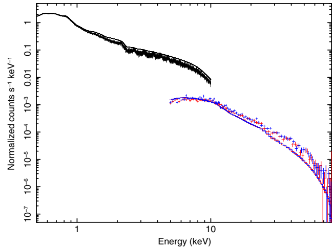
Fig. 4 SXI and HXI2 (identical to HXI1) spectra of the simulated X-ray background derived using skyback with the parameters displayed in Table 1 compared to a model that includes LHB, Halo, and the extragalactic spectrum from Ref. 29.
