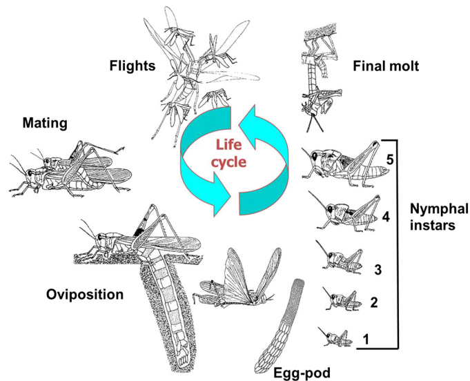
Fig. 9 Locust life cycle (modified from Ref. 32).
