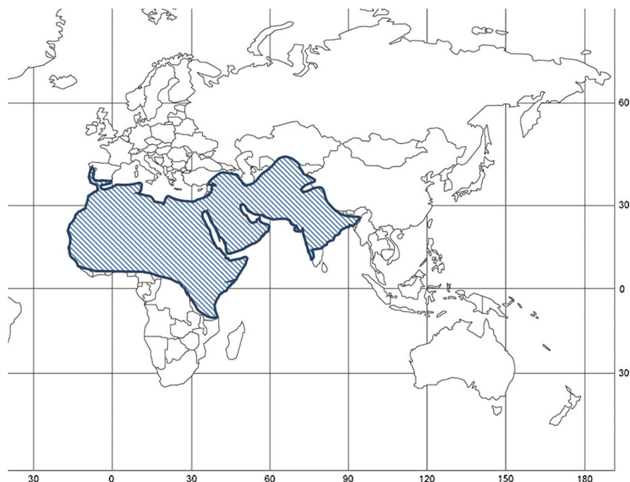
Fig. 6 Invasion area of the desert locust (modified from Ref. 3).
