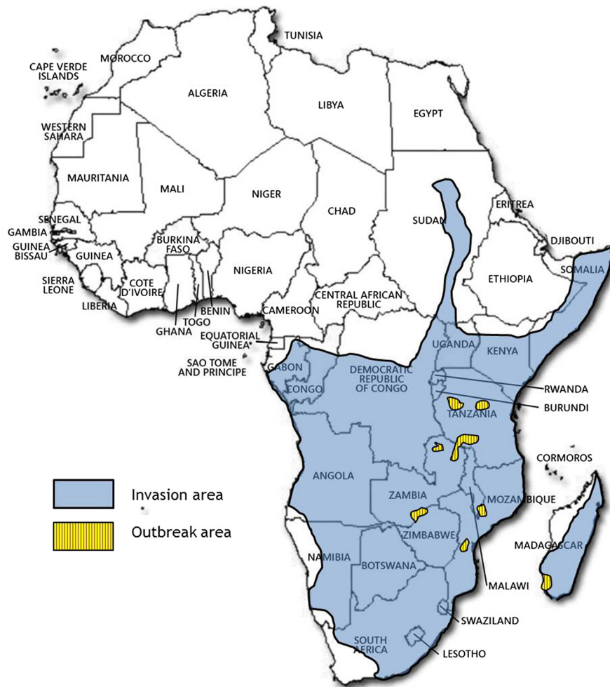
Fig. 29 Red locust distribution range (modified from Ref. 131).
