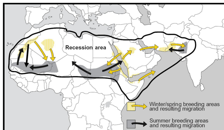
Fig. 12 Desert locust recession area with seasonal breeding zones and population movements between them (modified from Ref. 52).
