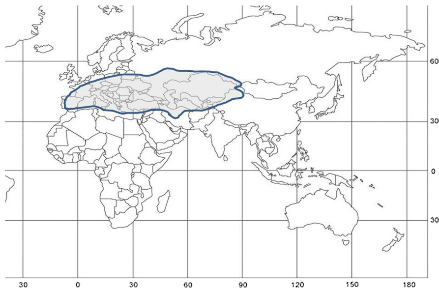
Fig. 25 Italian locust distribution range (modified from Ref. 32).
