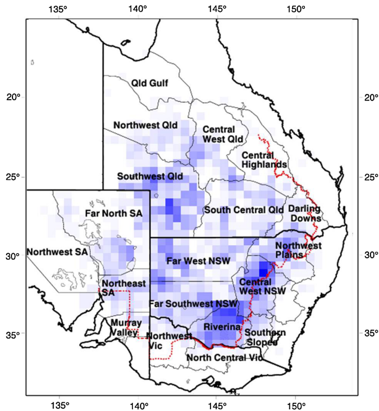
Fig. 16 Areas (shaded) of most frequent infestations of Australian plague locust in 1977–2008 (modified from Refs. 47 and 70).
