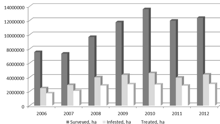
Fig. 8 Annual areas (in hectares) surveyed, infested and treated against the three locust species, C. italicus , D. maroccanus , and L. migratoria in five Central Asian countries (Kazakhstan, Kyrgyzstan, Tajikistan, Turkmenistan, and Uzbekistan) in 2006–2012. Data source: FAO “Locust Watch CCA” website ( http://www.fao.org/ag/locusts-CCA/en/index.html ).
