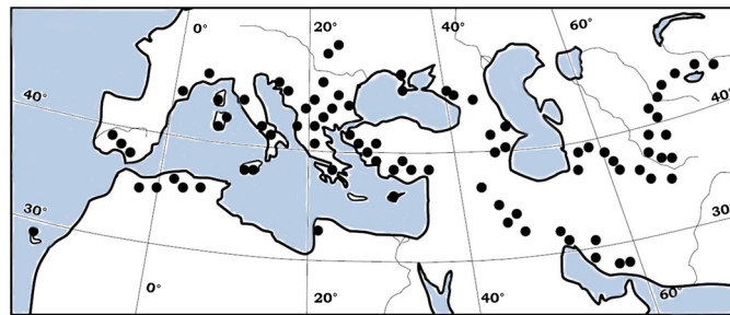
Fig. 22 Moroccan locust distribution range (modified from Ref. 32).
