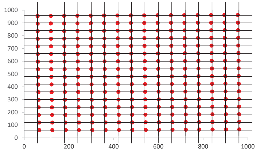
Figure 9. Coordinates of MINISTAR distorted pixel (red) compared to the ideal grid (in black) having the nodes in the ideal pixel center.
