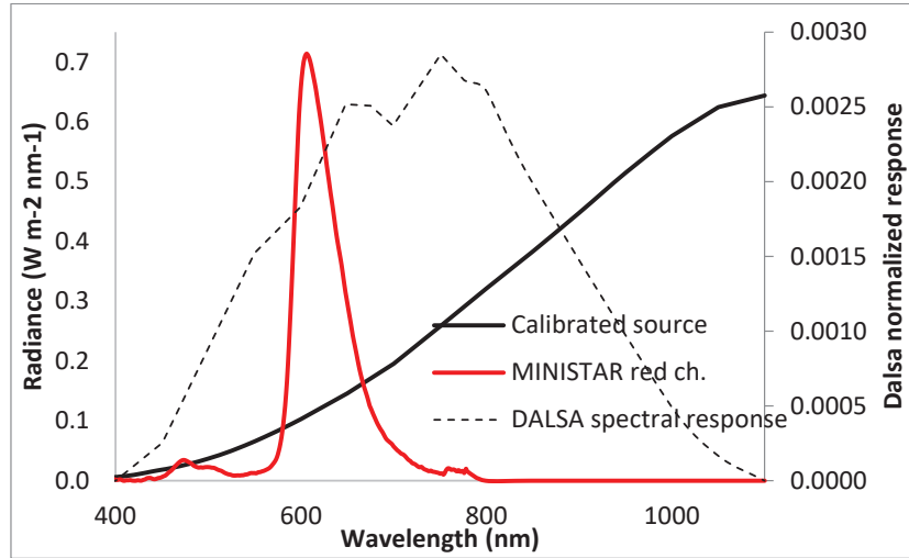
Figure 4. Spectral radiance of the MINISTAR channel used for the simulation (in our case the R channel) \langle R \rangle_{MS\Delta\lambda} (in red) and of the calibrated source HL-3P-INT-CAL equipped with Lambertian diffuser (in black), together with the DALSA 1M60 integrally normalized spectral response (dashed).
