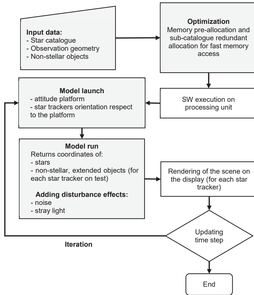
Figure 3. MINISTAR software scheme showing the optimization phase of the mathematical model (at allocation time) followed by the model launch. This structure increases computational speed.
