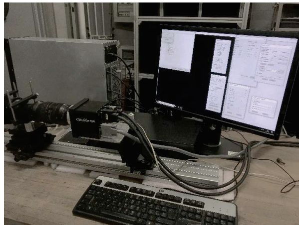
Figure 4. MINISTAR prototype during laboratory tests. On the left, the prototype faced to the objective and the camera used for the test (DALSA, 1M60 model).
