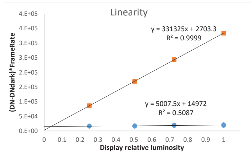
Figure 6. Verification of linearity in radiometric response in DN of the MINISTAR display as a function of its relative luminosity.
