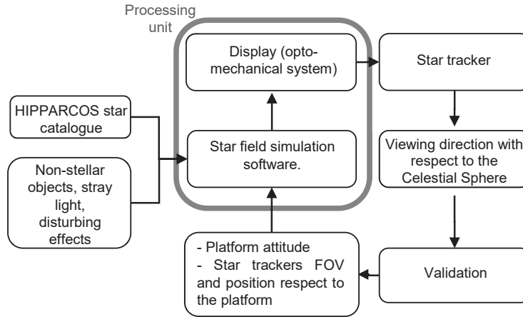
Figure 1. Block diagram of the MINISTAR system showing the main elements of a simulation in closed-loop configuration for validation of the star tracker under test.
