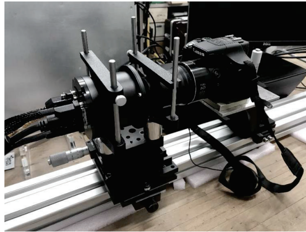
Figure 8. Laboratory setup for geometric calibration: MINISTAR (left) is faced to Canon SX60 HS camera.
