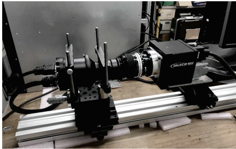
Figure 5. Setup for radiometric calibration: MINISTAR is faced to the NIKON objective coupled to the DALSA camera.
