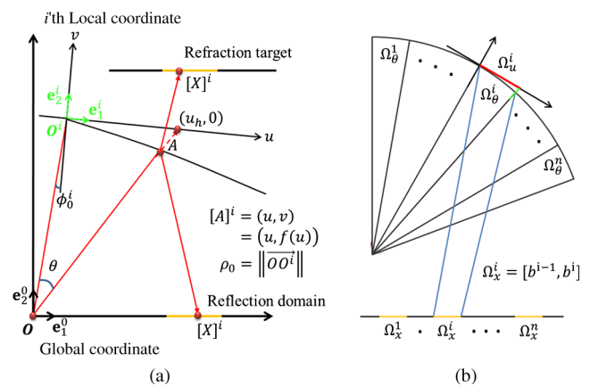
Fig. 1 (a) Global coordinate system: origin ( \mathbf{O} ) locates at light source with basis vectors \{\mathbf{e}_1^0, \mathbf{e}_2^0\} . Local i 'th coordinate system: origin ( \mathbf{O}^i ) locates at freeform surface with local basis vectors \{\mathbf{e}_1^i, \mathbf{e}_2^i\} . The angles \theta and \phi_0^i are the angle of \overrightarrow{\mathbf{O}\mathbf{O}^i} with \overrightarrow{\mathbf{O}\mathbf{A}} and \mathbf{e}_2^i , respectively. A 1-D freeform model assumes that the global coordinate and local coordinate are coplanar. (b) Partitioning \Omega_\theta and \Omega_x into n subdomain \Omega_\theta^i and \Omega_x^i for i = 1, 2, \dots, n is based on equal flux theory. Computation domain \Omega_u^i that unifying variable u and x into local variable u is mapped from subdomain \Omega_\theta^i and \Omega_x^i .
