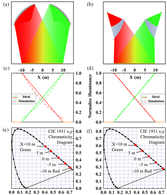
Fig. 5 (a) and (b) Layout of the freeform surface reflector and refractor is designed for chromatic varying illuminance. The CIE chromatic of two point sources is red (x, y) = (0.73, 0.27) and green (x, y) = (0.38, 0.62) . (c) and (d) Comparison of illuminance pattern by the constructed freeform surface (dash line) and that with ideally linear shape (solid line). The nonuniformity with the ideal linear case was well controlled within 5.58% RMS and 1.52% RMS in reflection case and refraction case, respectively. (e) and (f) Five sampling points along x -direction ( -10, -5, 0, 5, 10 m) exhibit a linearly chromatic shift in CIE 1931 x, y chromaticity coordinate in both case.
